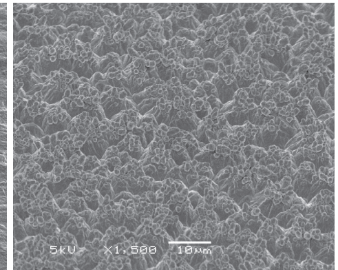
Treated Matte Side H oz. /18 µm (1500x)
